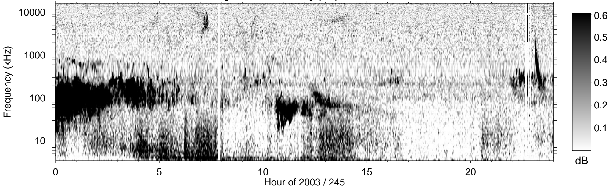
RPWS [ABCH1H2/Ex] (-B) 2003/09/02
