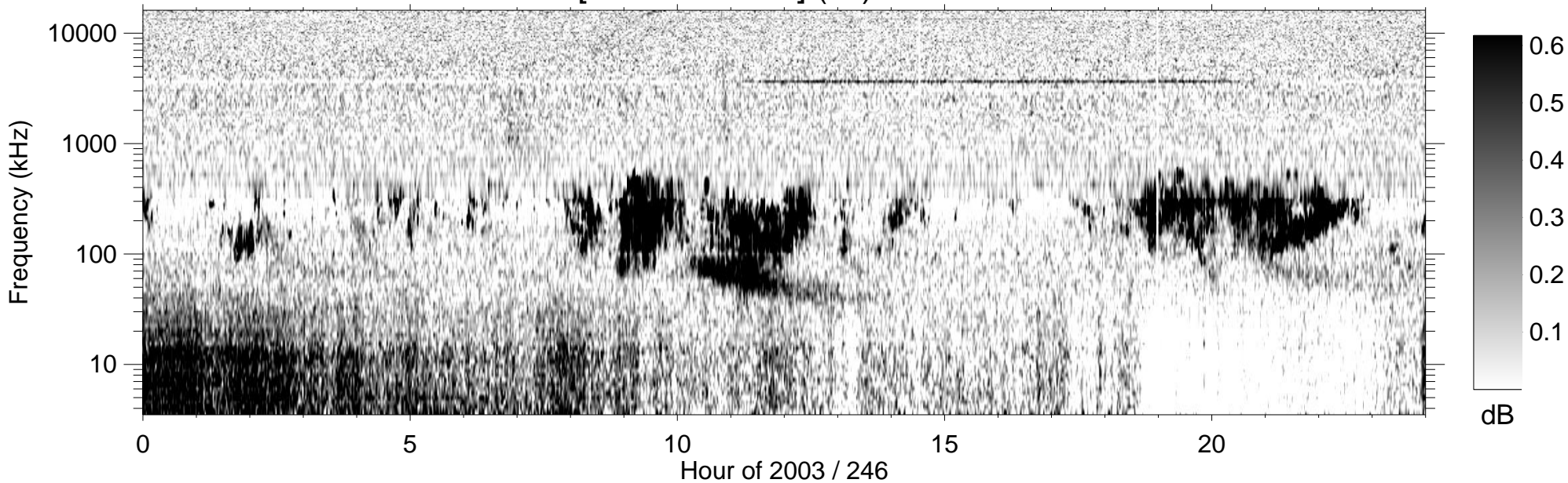
RPWS [ABCH1H2/Ex] (-B) 2003/09/03
