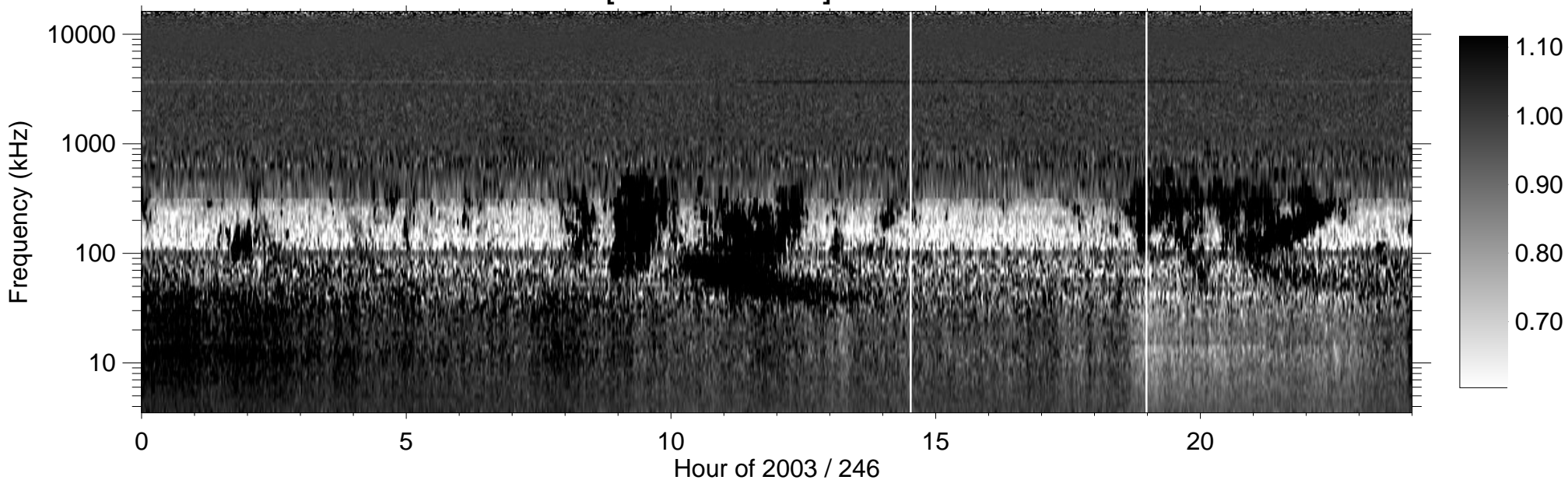
RPWS [ABCH1H2/Ex] (-B) 2003/09/03
