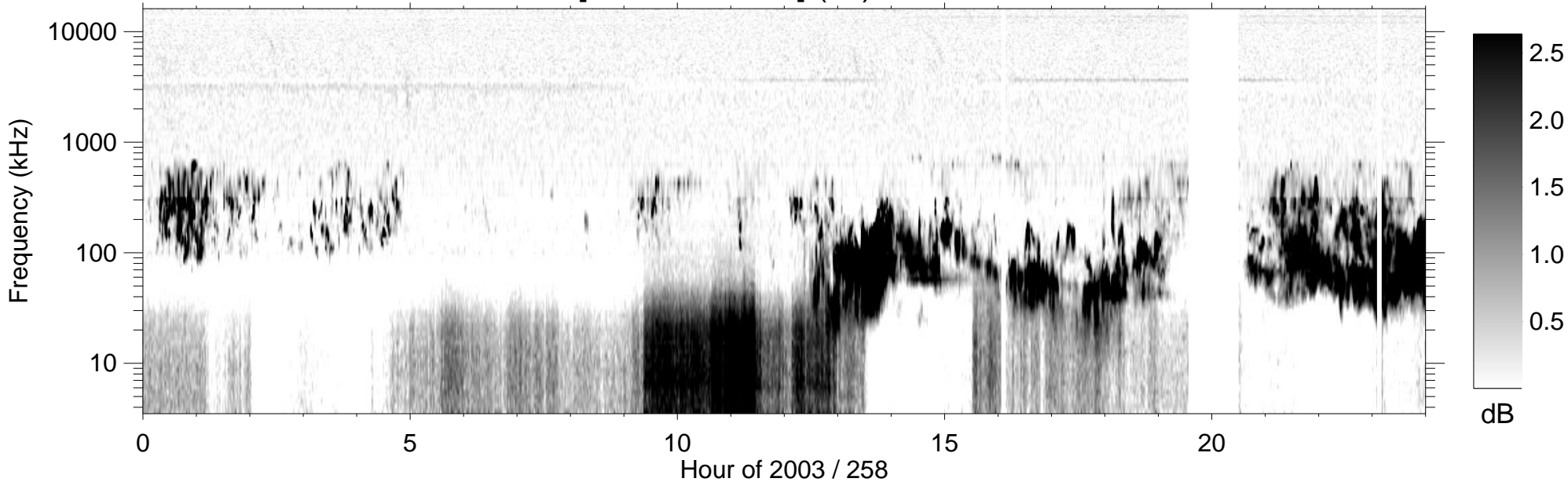
RPWS [ABCH1H2/Ex] (-B) 2003/09/15
