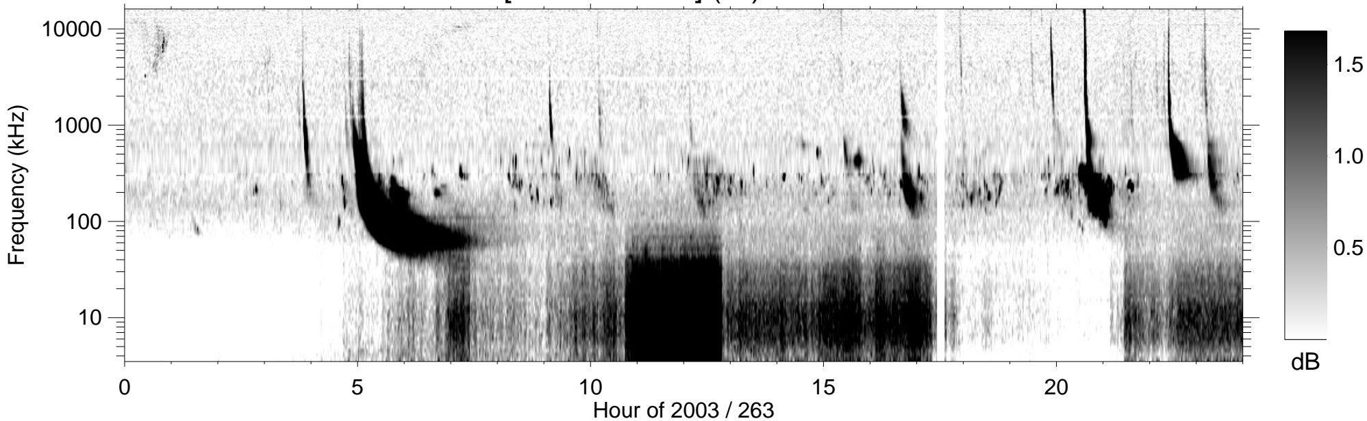
RPWS [ABCH1H2/Ex] (-B) 2003/09/20
