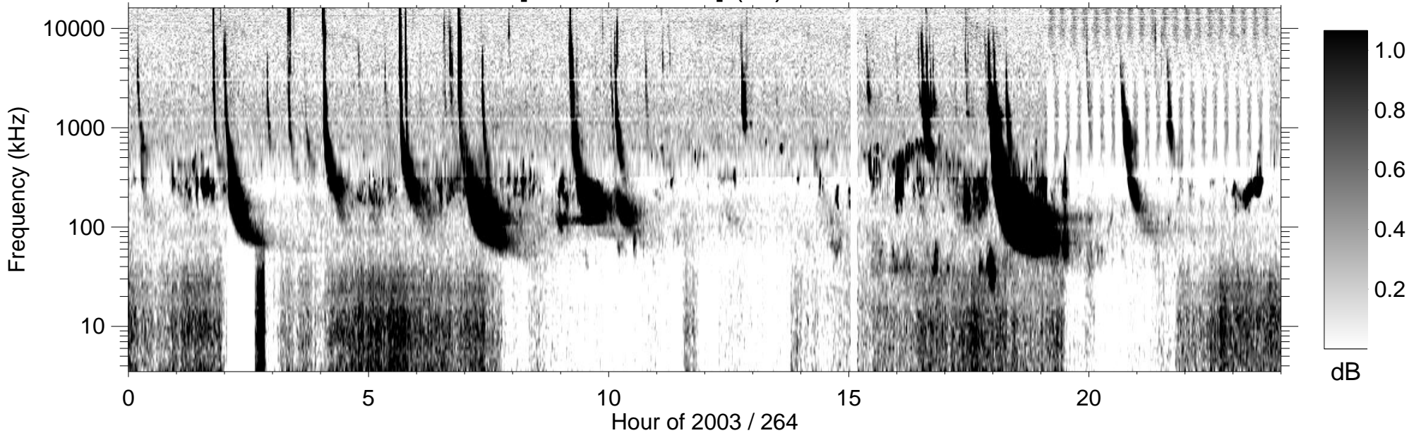
RPWS [ABCH1H2/Ex] (-B) 2003/09/21
