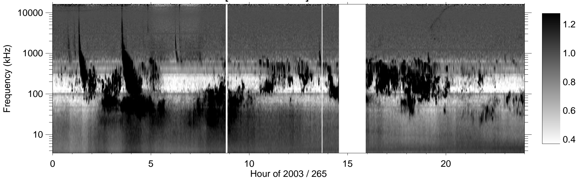
RPWS [ABCH1H2/Ex] (-B) 2003/09/22
