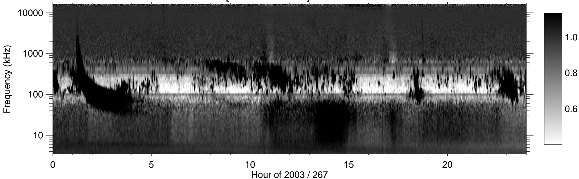
RPWS [ABCH1H2/Ex] (-B) 2003/09/24
