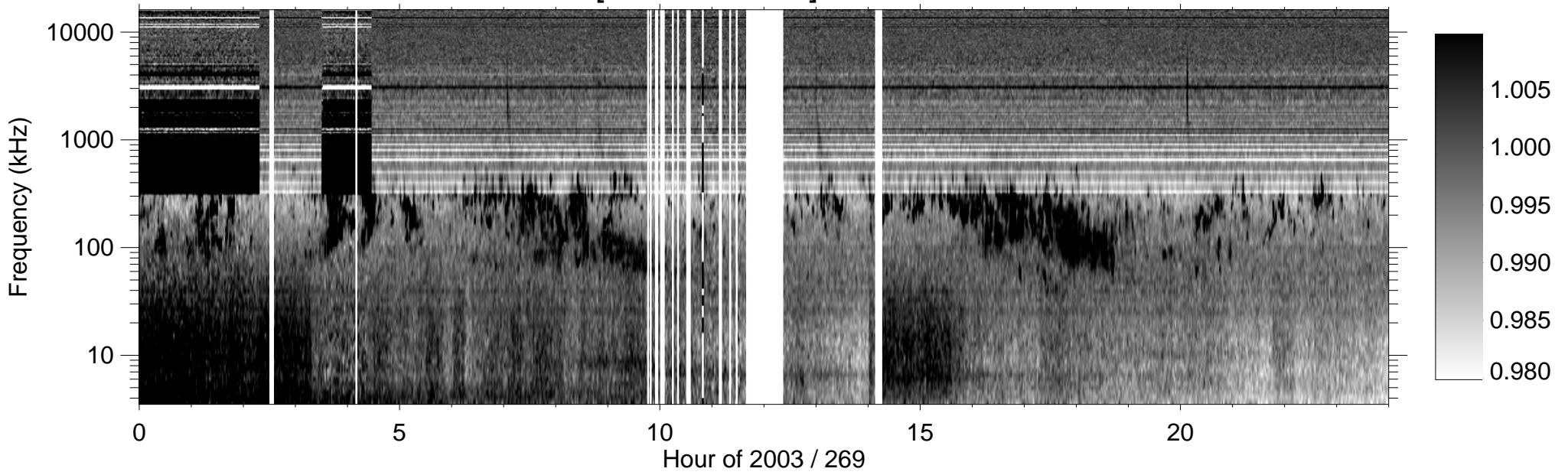
RPWS [ABCH1H2/Ex] (-B) 2003/09/26
