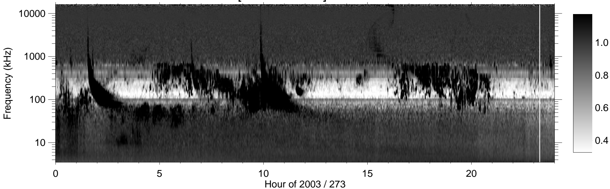
RPWS [ABCH1H2/Ex] (-B) 2003/09/30
