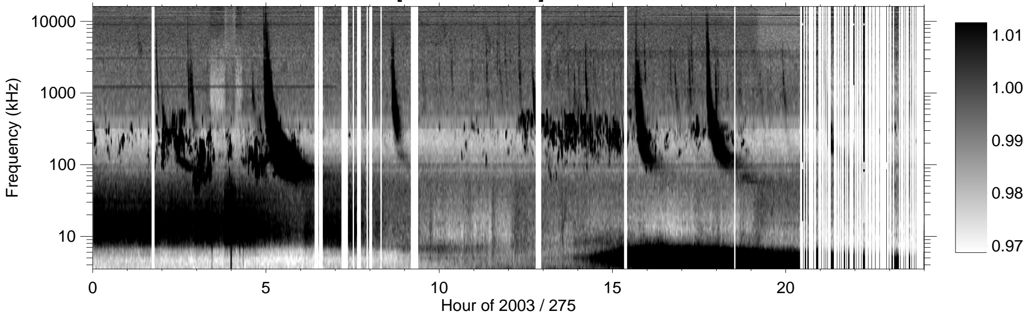
RPWS [ABCH1H2/Ex] (-B) 2003/10/02
