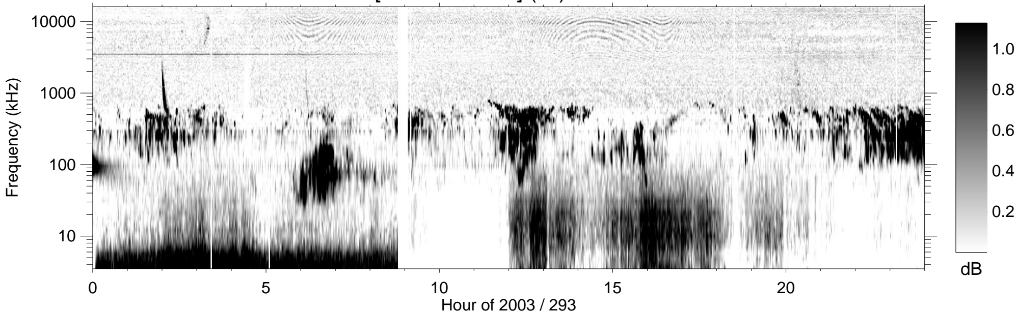
RPWS [ABCH1H2/Ex] (-B) 2003/10/20
