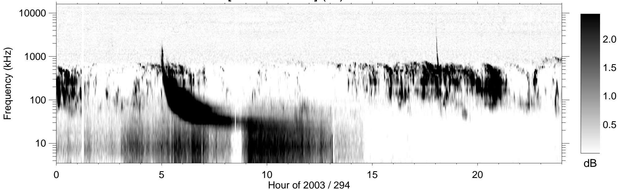
RPWS [ABCH1H2/Ex] (-B) 2003/10/21
