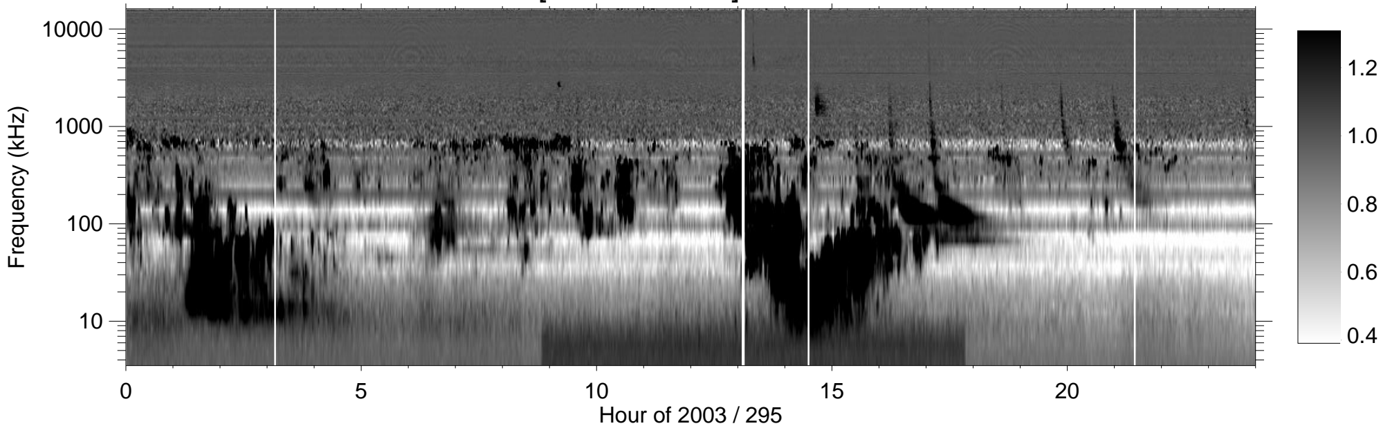
RPWS [ABCH1H2/Ex] (-B) 2003/10/22
