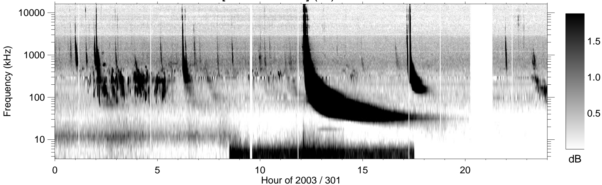
RPWS [ABCH1H2/Ex] (-B) 2003/10/28
