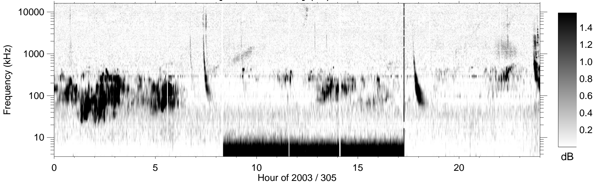
RPWS [ABCH1H2/Ex] (-B) 2003/11/01
