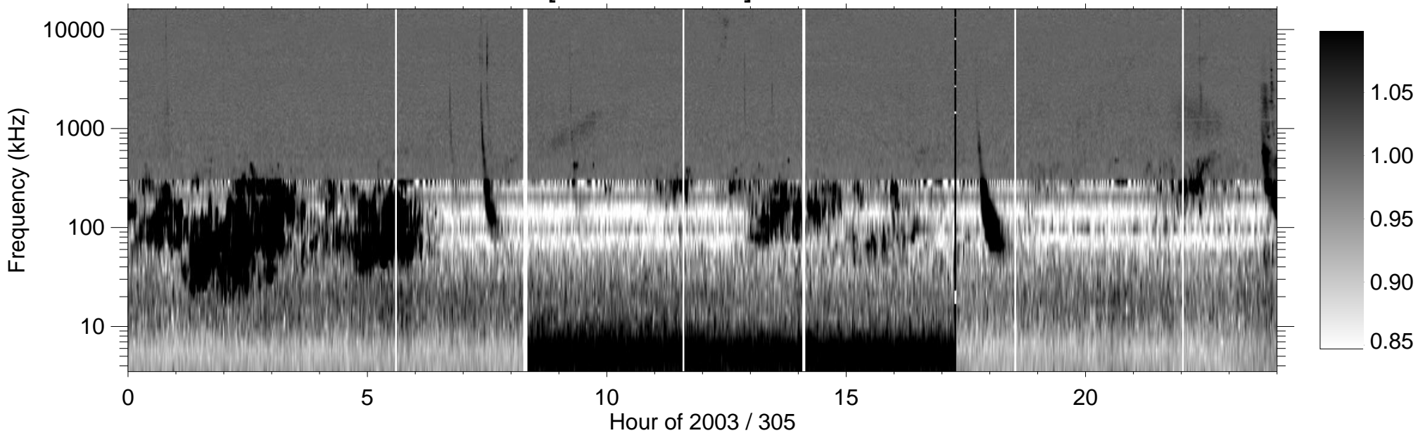
RPWS [ABCH1H2/Ex] (-B) 2003/11/01
