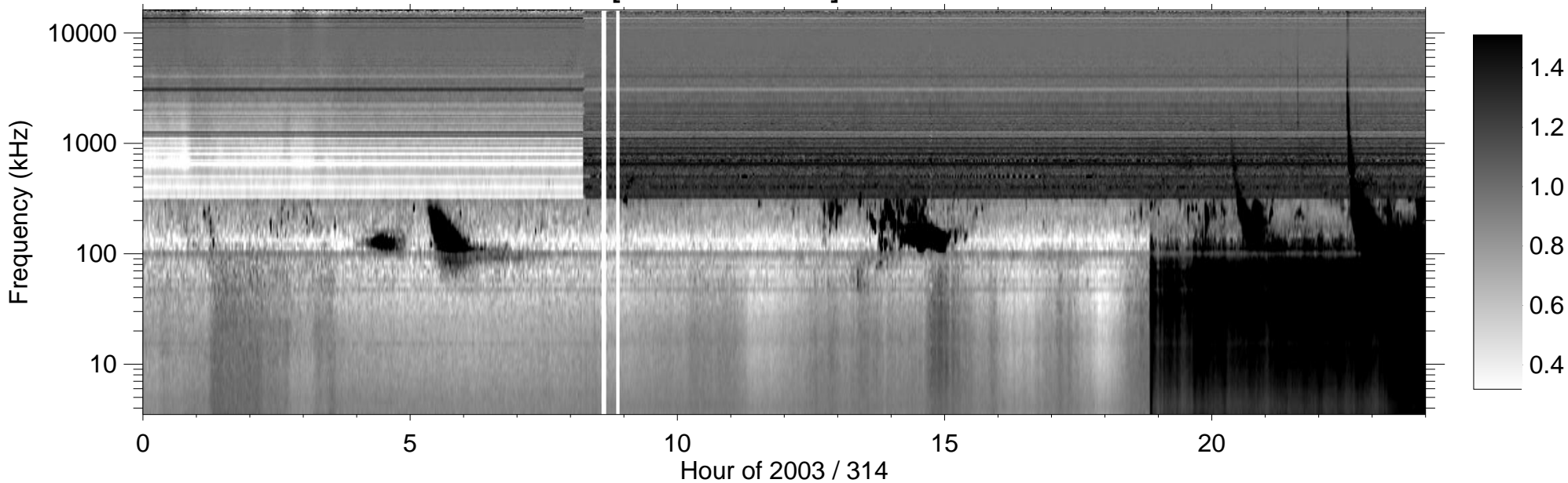
RPWS [ABCH1H2/Ex] (-B) 2003/11/10
