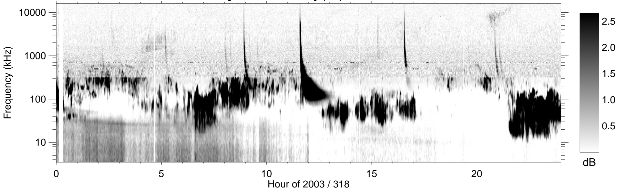
RPWS [ABCH1H2/Ex] (-B) 2003/11/14
