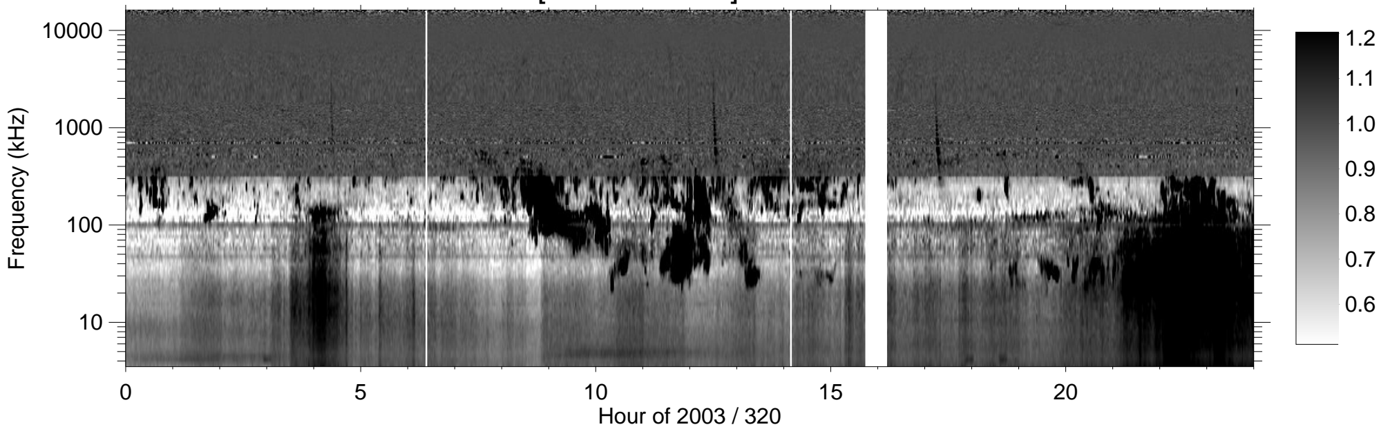
RPWS [ABCH1H2/Ex] (-B) 2003/11/16
