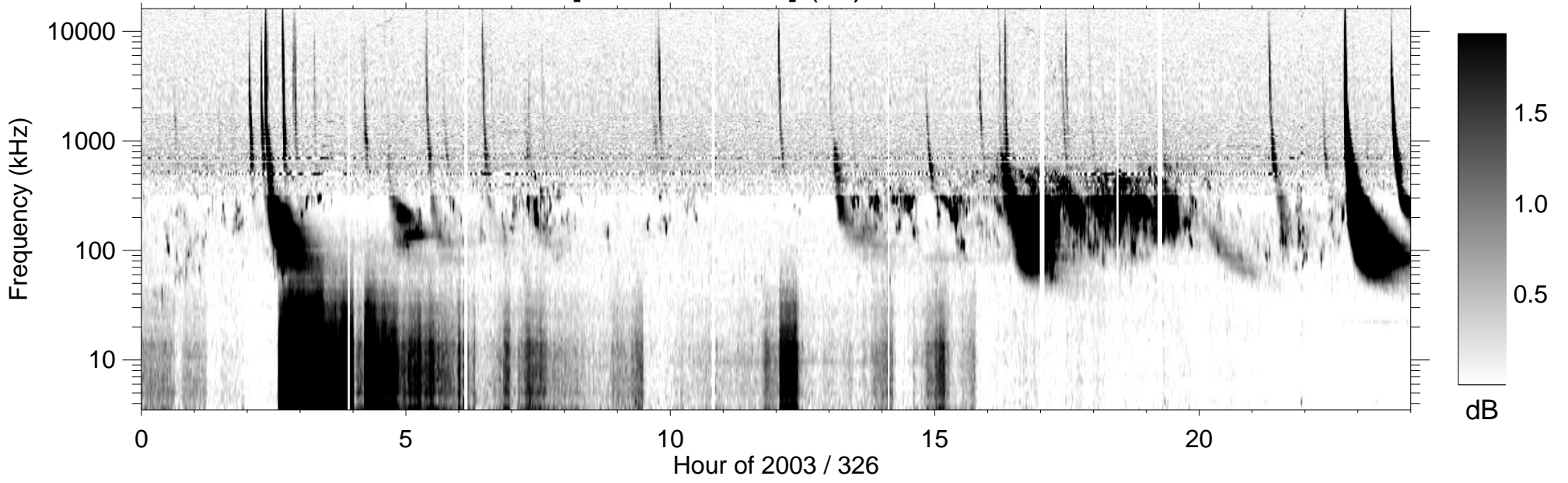
RPWS [ABCH1H2/Ex] (-B) 2003/11/22
