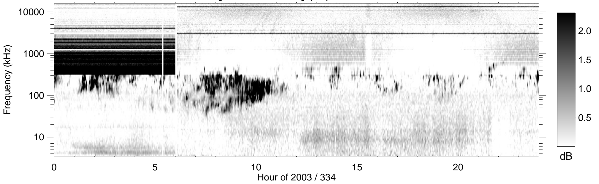
RPWS [ABCH1H2/Ex] (-B) 2003/11/30
