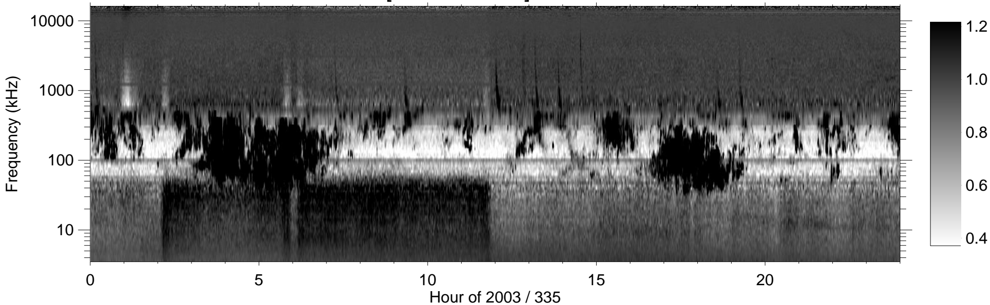
RPWS [ABCH1H2/Ex] (-B) 2003/12/01
