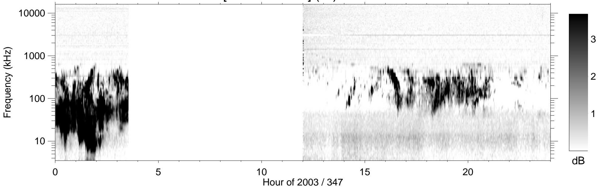
RPWS [ABCH1H2/Ex] (-B) 2003/12/13
