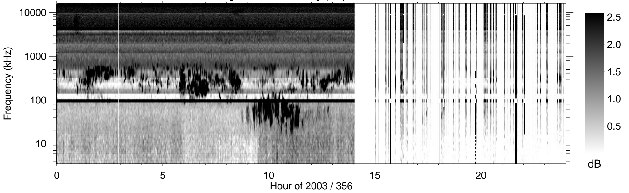
RPWS [ABCH1H2/Ex] (-B) 2003/12/22
