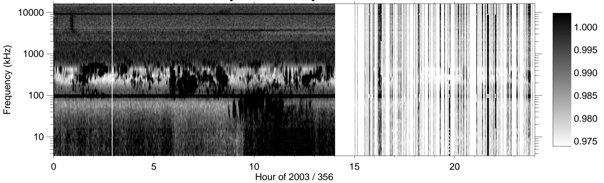
RPWS [ABCH1H2/Ex] (-B) 2003/12/22
