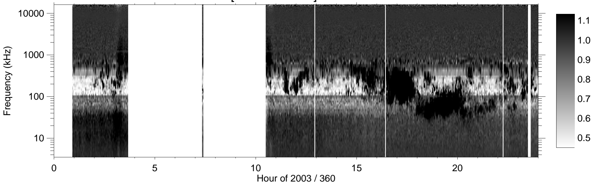
RPWS [ABCH1H2/Ex] (-B) 2003/12/26
