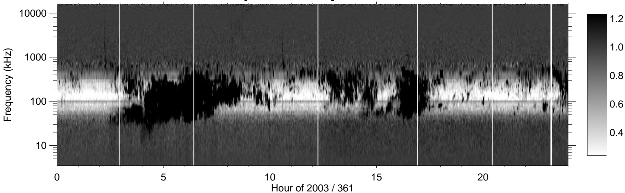
RPWS [ABCH1H2/Ex] (-B) 2003/12/27
