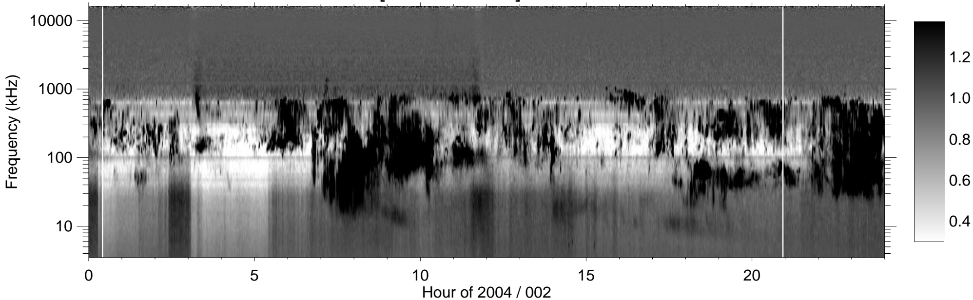
RPWS [ABCH1H2/Ex] (-B) 2004/01/02
