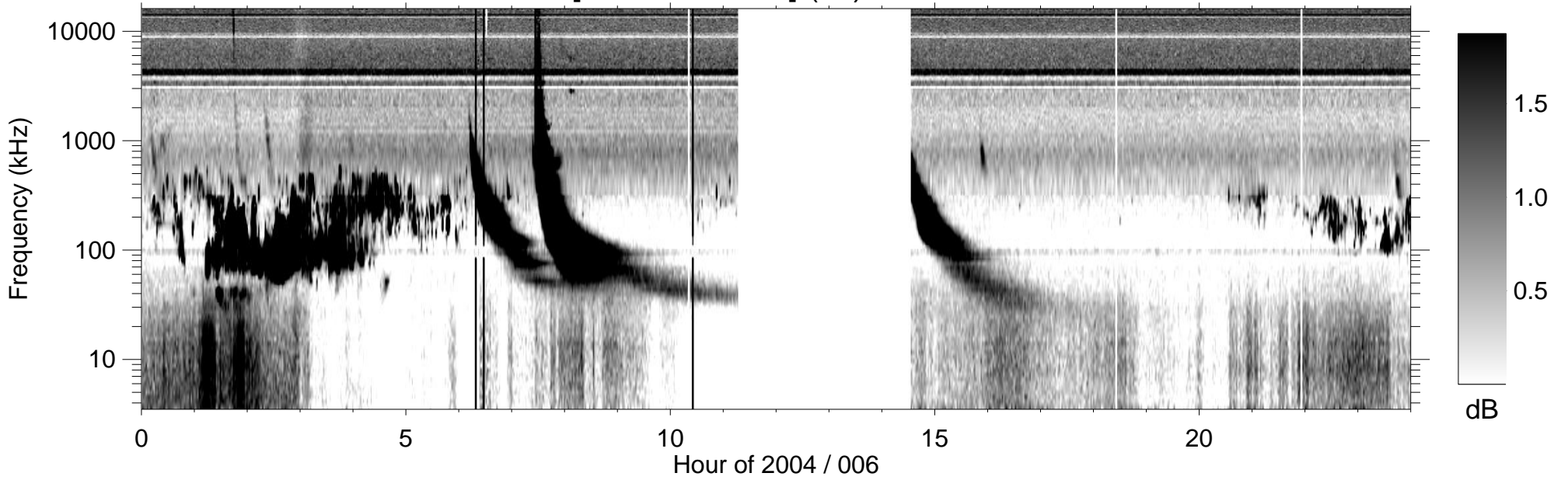
RPWS [ABCH1H2/Ex] (-B) 2004/01/06
