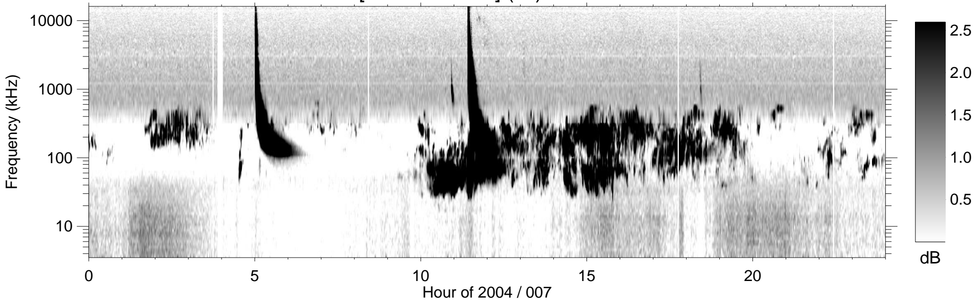
RPWS [ABCH1H2/Ex] (-B) 2004/01/07
