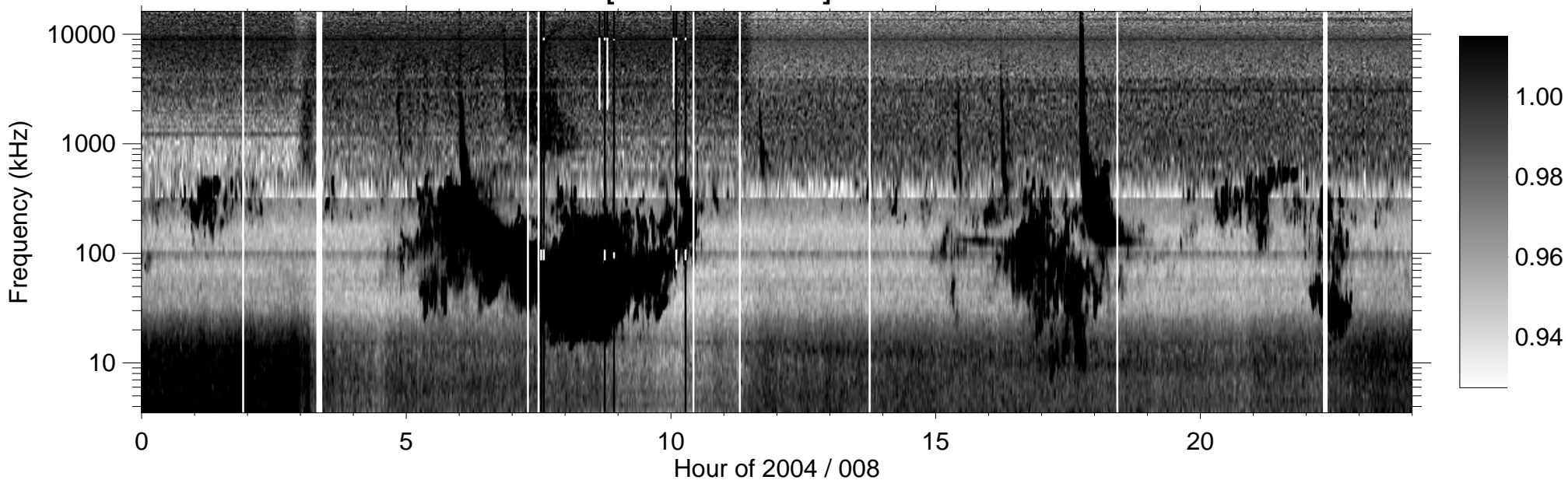
RPWS [ABCH1H2/Ex] (-B) 2004/01/08
