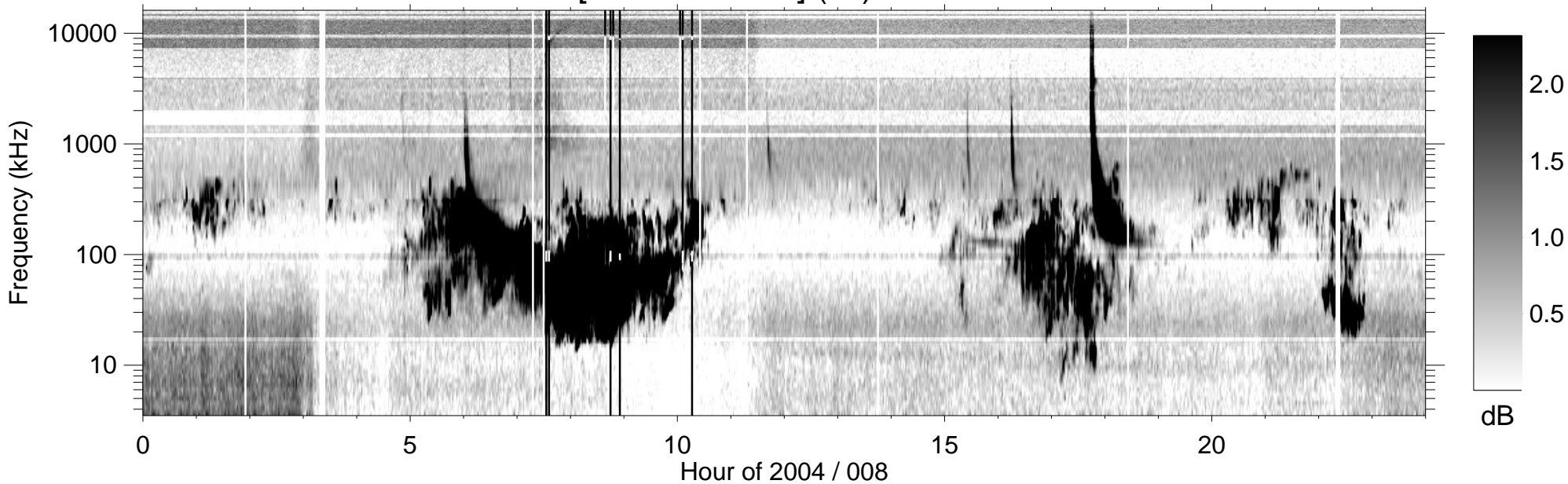
RPWS [ABCH1H2/Ex] (-B) 2004/01/08
