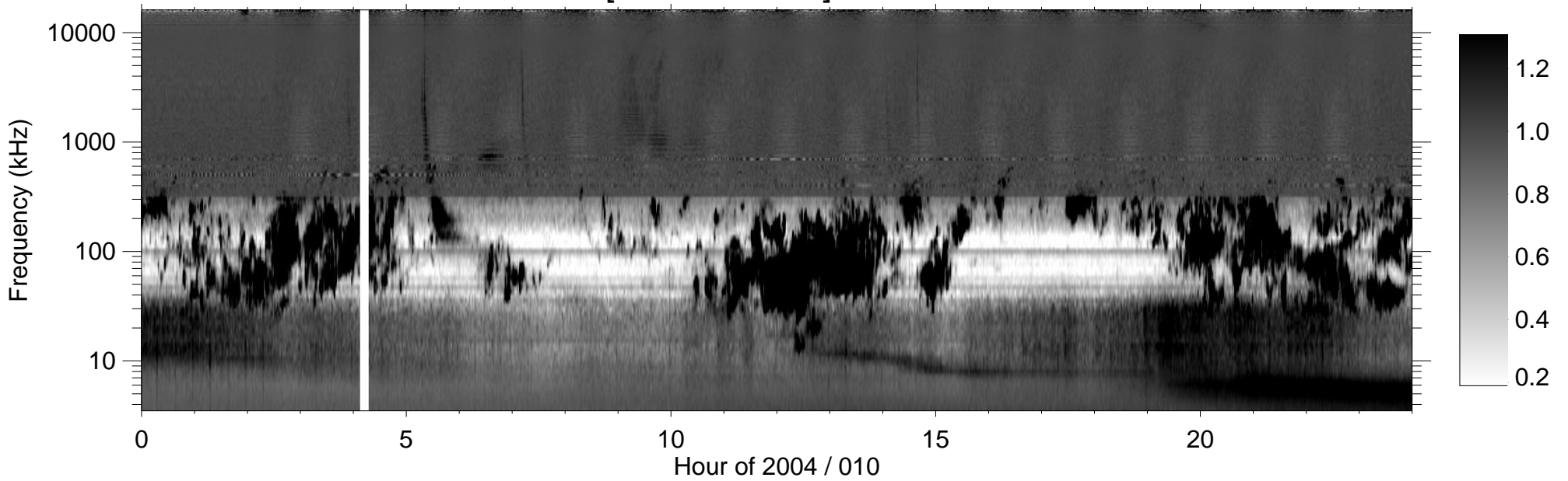
RPWS [ABCH1H2/Ex] (-B) 2004/01/10
