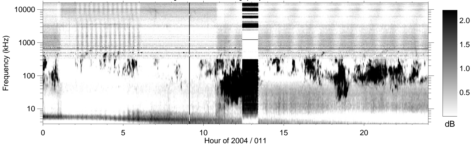
RPWS [ABCH1H2/Ex] (-B) 2004/01/11
