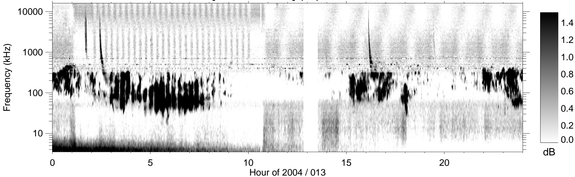
RPWS [ABCH1H2/Ex] (-B) 2004/01/13
