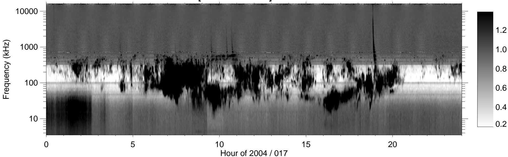
RPWS [ABCH1H2/Ex] (-B) 2004/01/17
