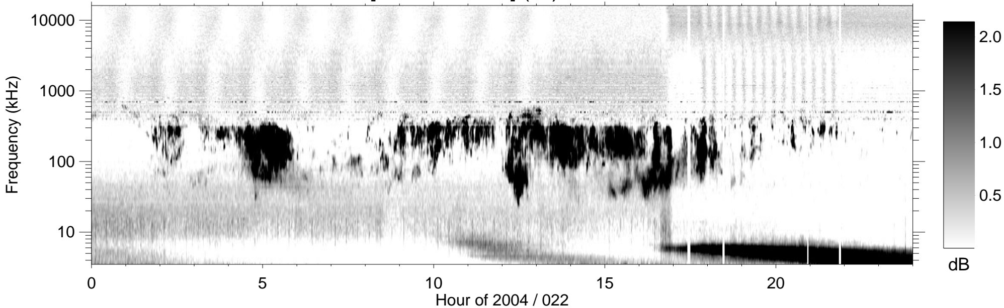
RPWS [ABCH1H2/Ex] (-B) 2004/01/22
