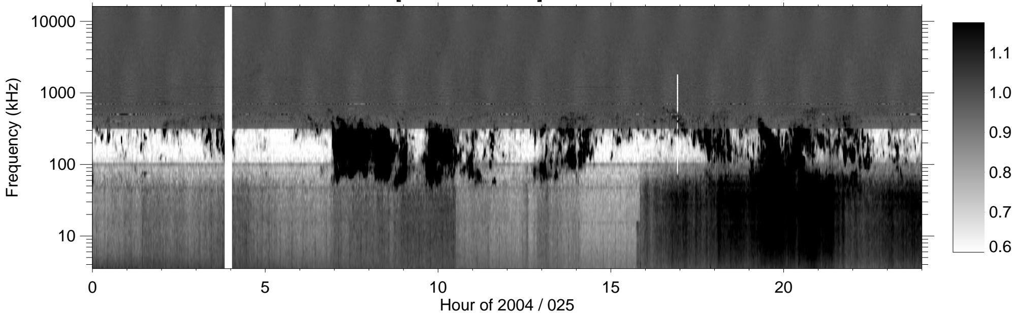
RPWS [ABCH1H2/Ex] (-B) 2004/01/25
