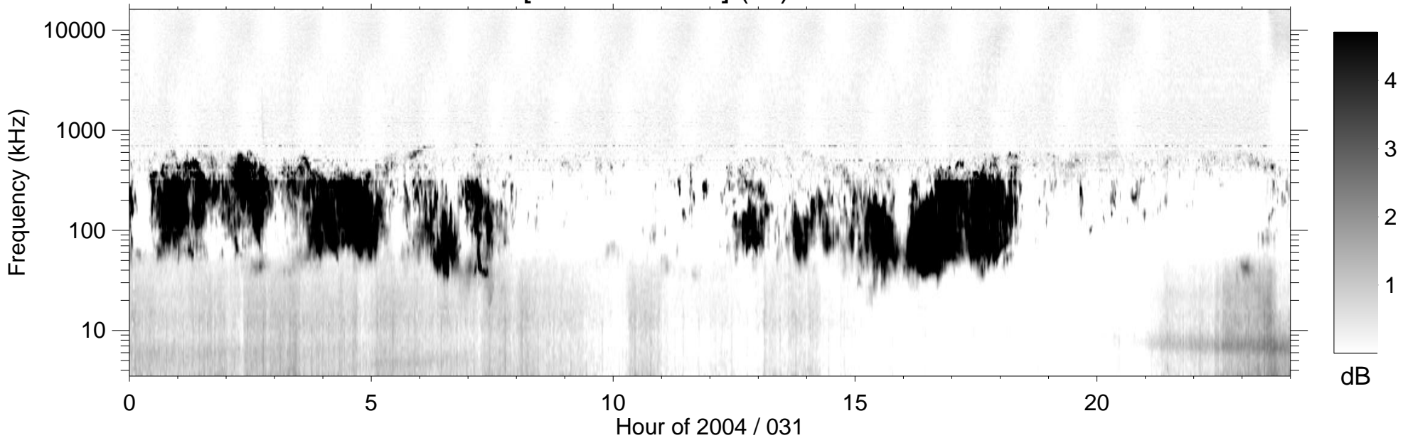
RPWS [ABCH1H2/Ex] (-B) 2004/01/31
