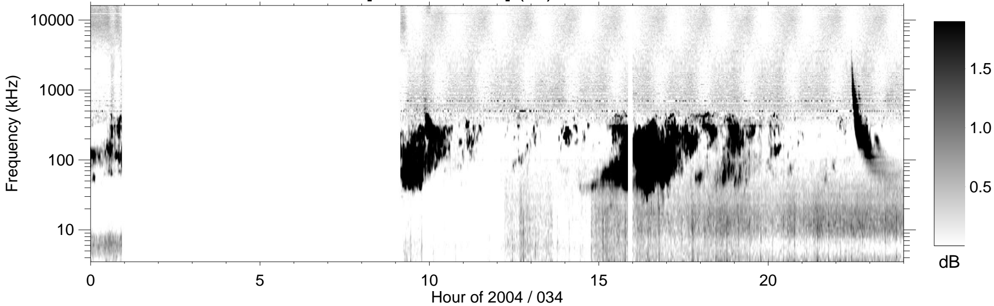
RPWS [ABCH1H2/Ex] (-B) 2004/02/03
