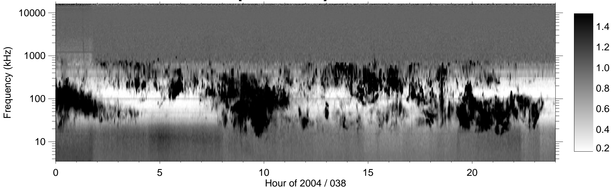
RPWS [ABCH1H2/Ex] (-B) 2004/02/07
