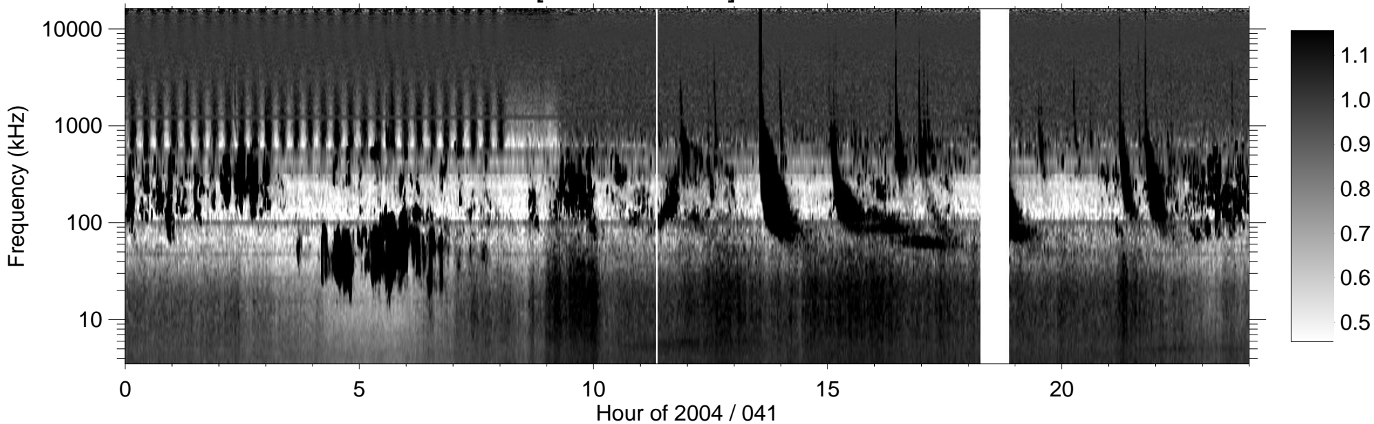
RPWS [ABCH1H2/Ex] (-B) 2004/02/10
