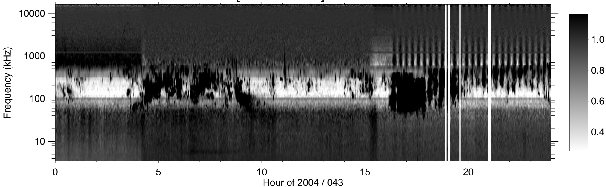
RPWS [ABCH1H2/Ex] (-B) 2004/02/12
