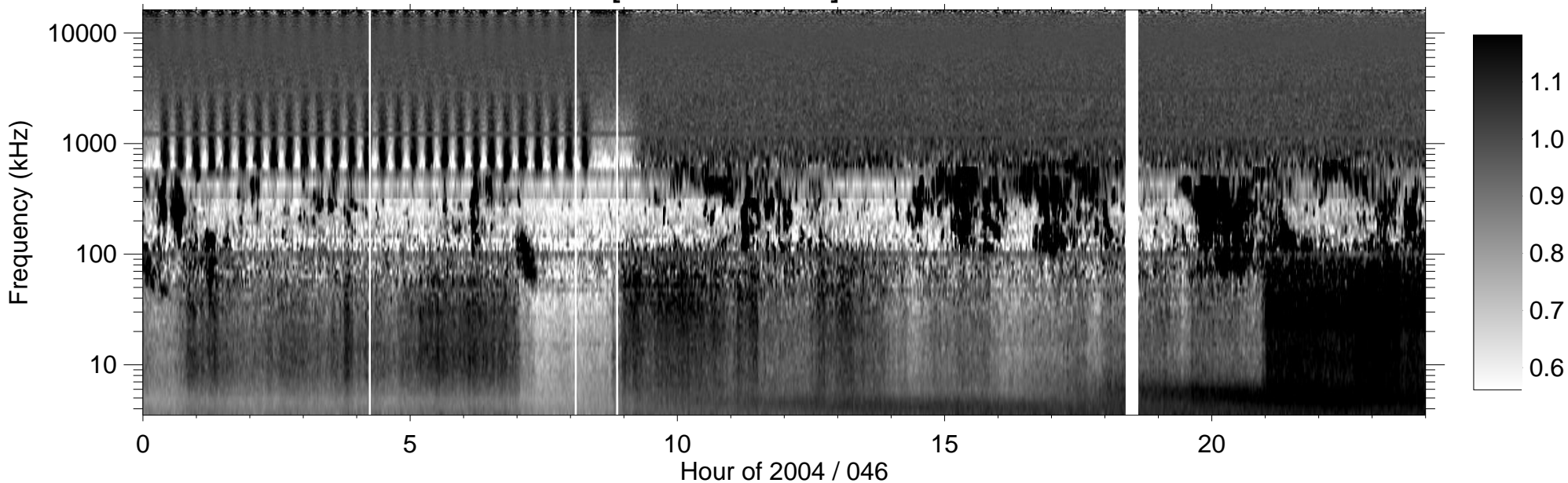
RPWS [ABCH1H2/Ex] (-B) 2004/02/15
