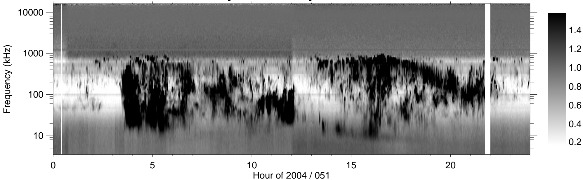
RPWS [ABCH1H2/Ex] (-B) 2004/02/20
