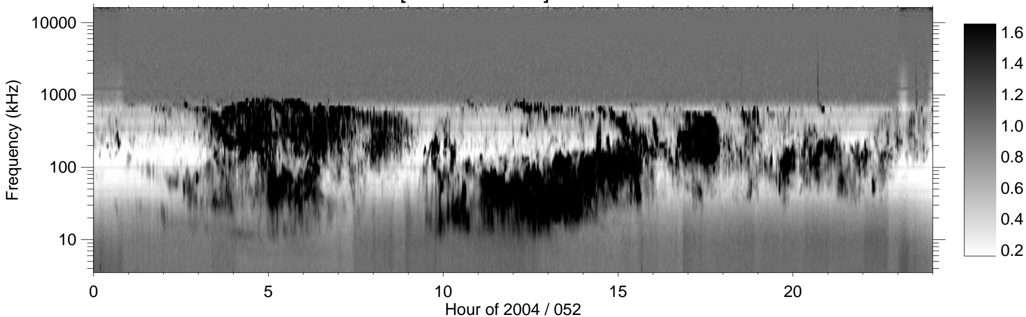
RPWS [ABCH1H2/Ex] (-B) 2004/02/21
