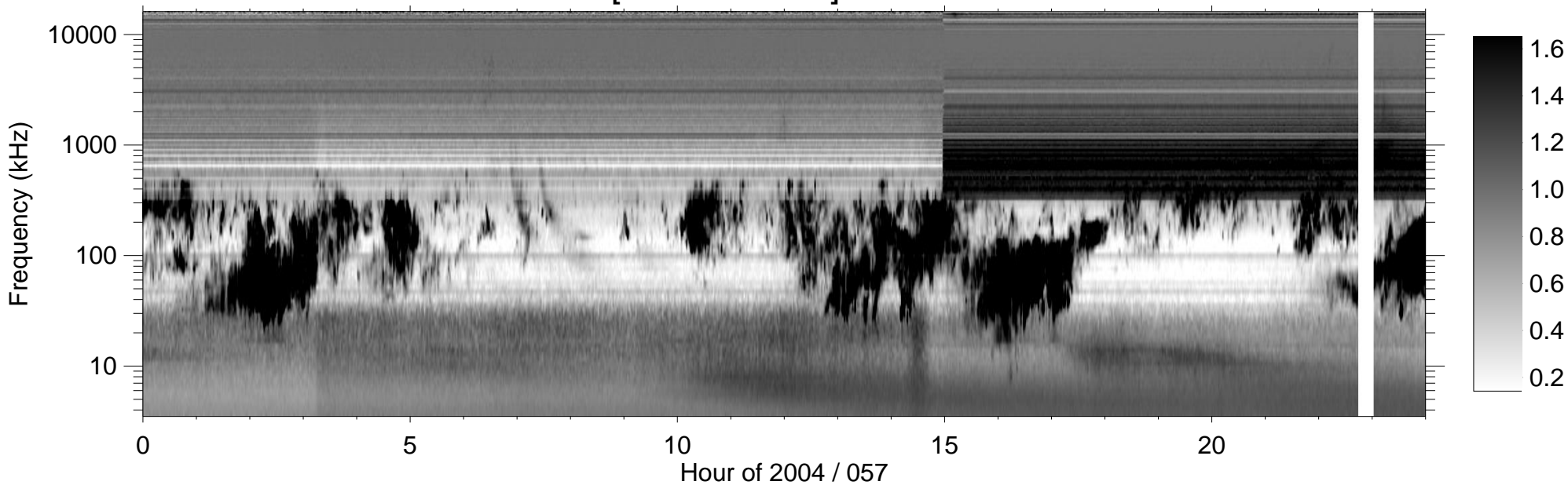
RPWS [ABCH1H2/Ex] (-B) 2004/02/26
