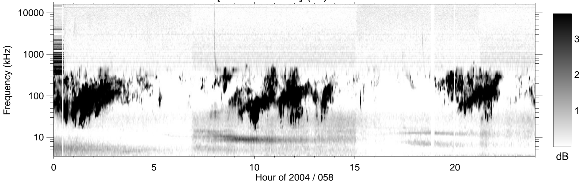
RPWS [ABCH1H2/Ex] (-B) 2004/02/27
