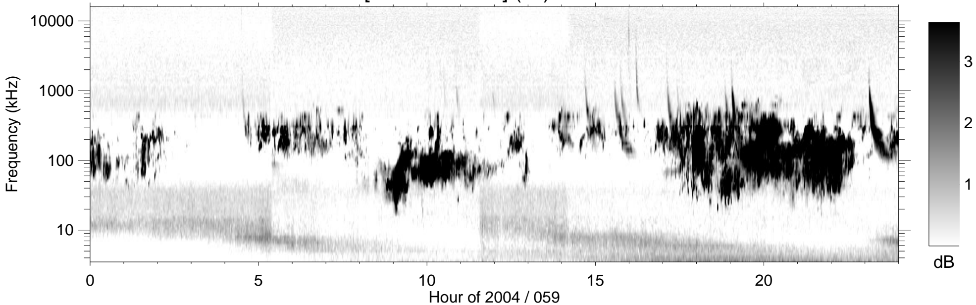
RPWS [ABCH1H2/Ex] (-B) 2004/02/28
