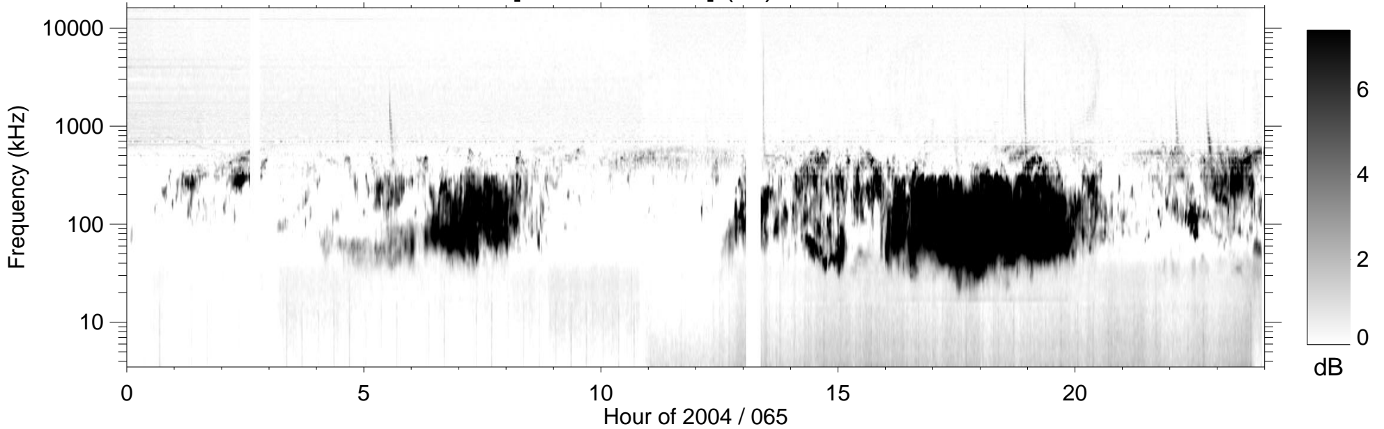
RPWS [ABCH1H2/Ex] (-B) 2004/03/05
