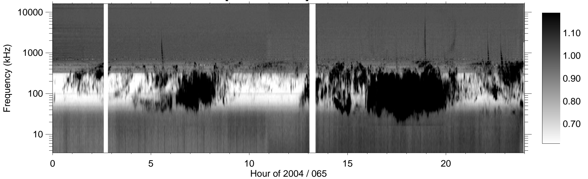
RPWS [ABCH1H2/Ex] (-B) 2004/03/05
