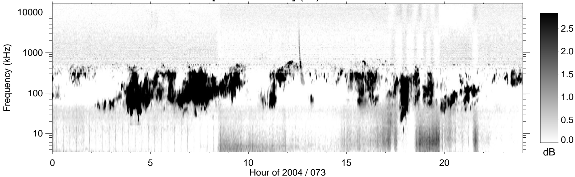
RPWS [ABCH1H2/Ex] (-B) 2004/03/13
