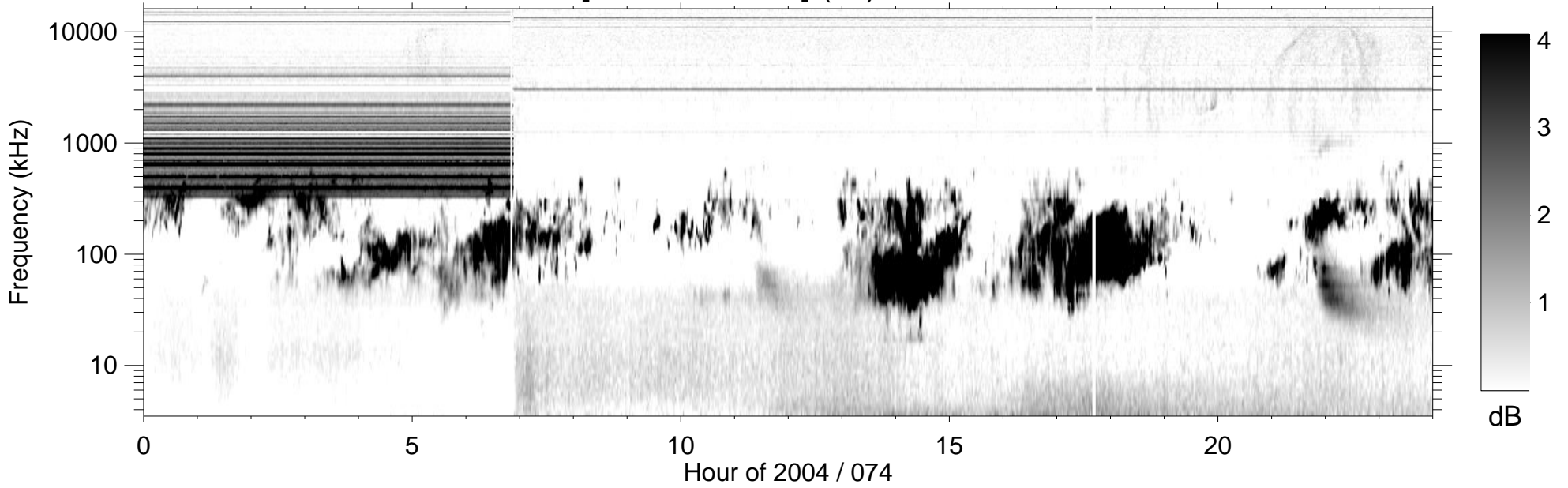
RPWS [ABCH1H2/Ex] (-B) 2004/03/14
