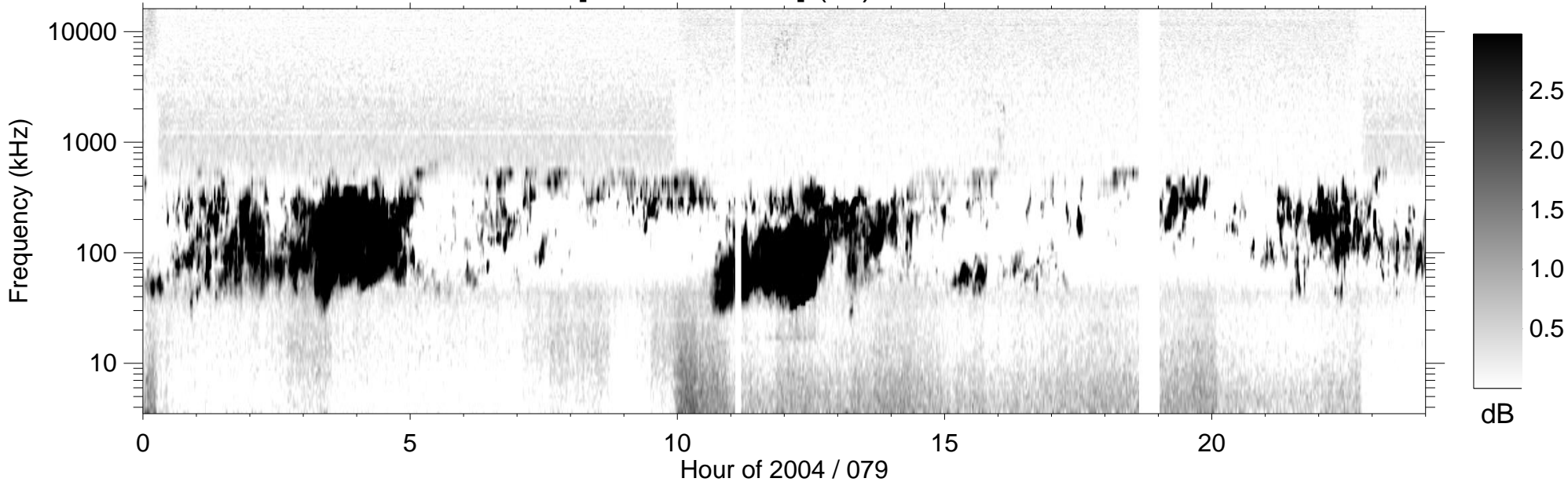
RPWS [ABCH1H2/Ex] (-B) 2004/03/19
